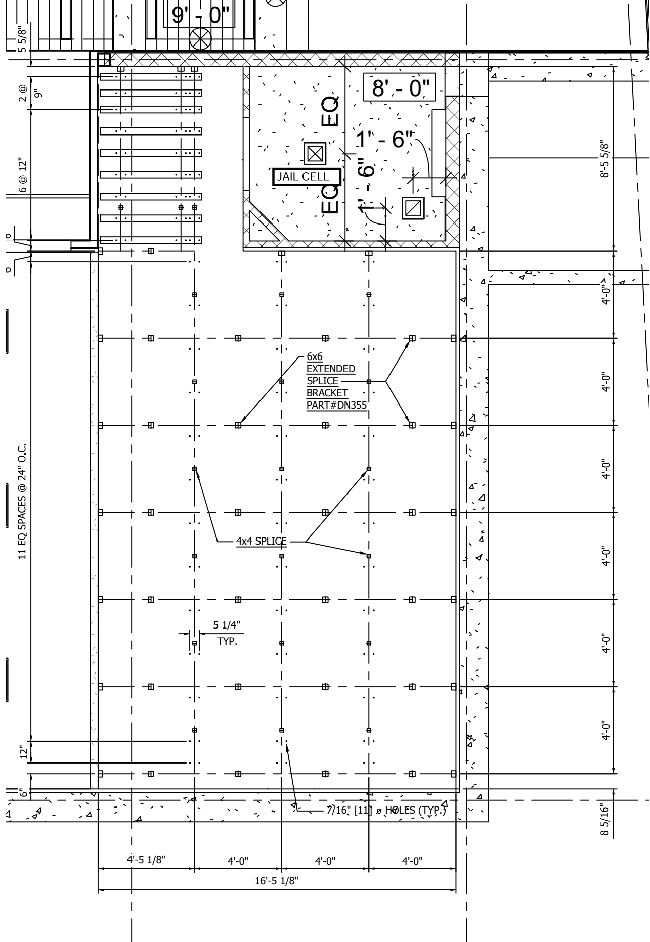
1 ENTRY LEVEL- BDLG A HANGER ROD LAYOUT
